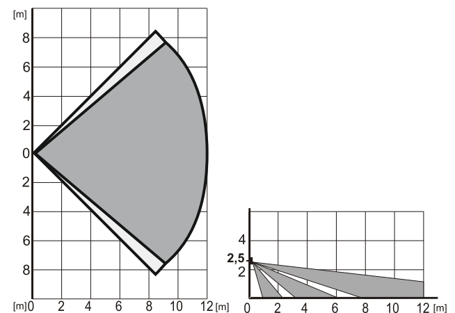
Fig 2: Detection characteristics
