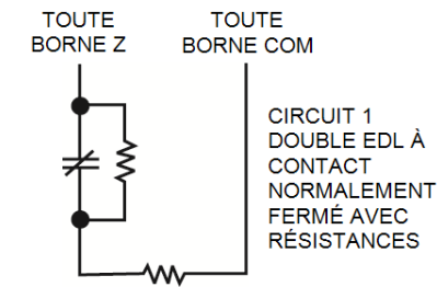
Figure 1-4 Câblage DEDL
